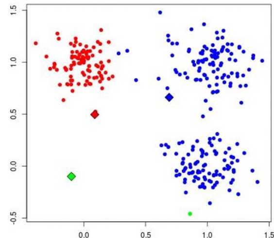
Update Cluster Assignments
