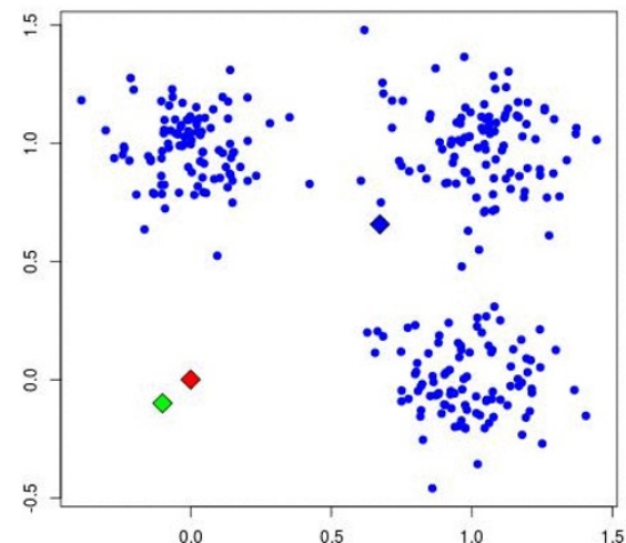
Update Cluster Centers
